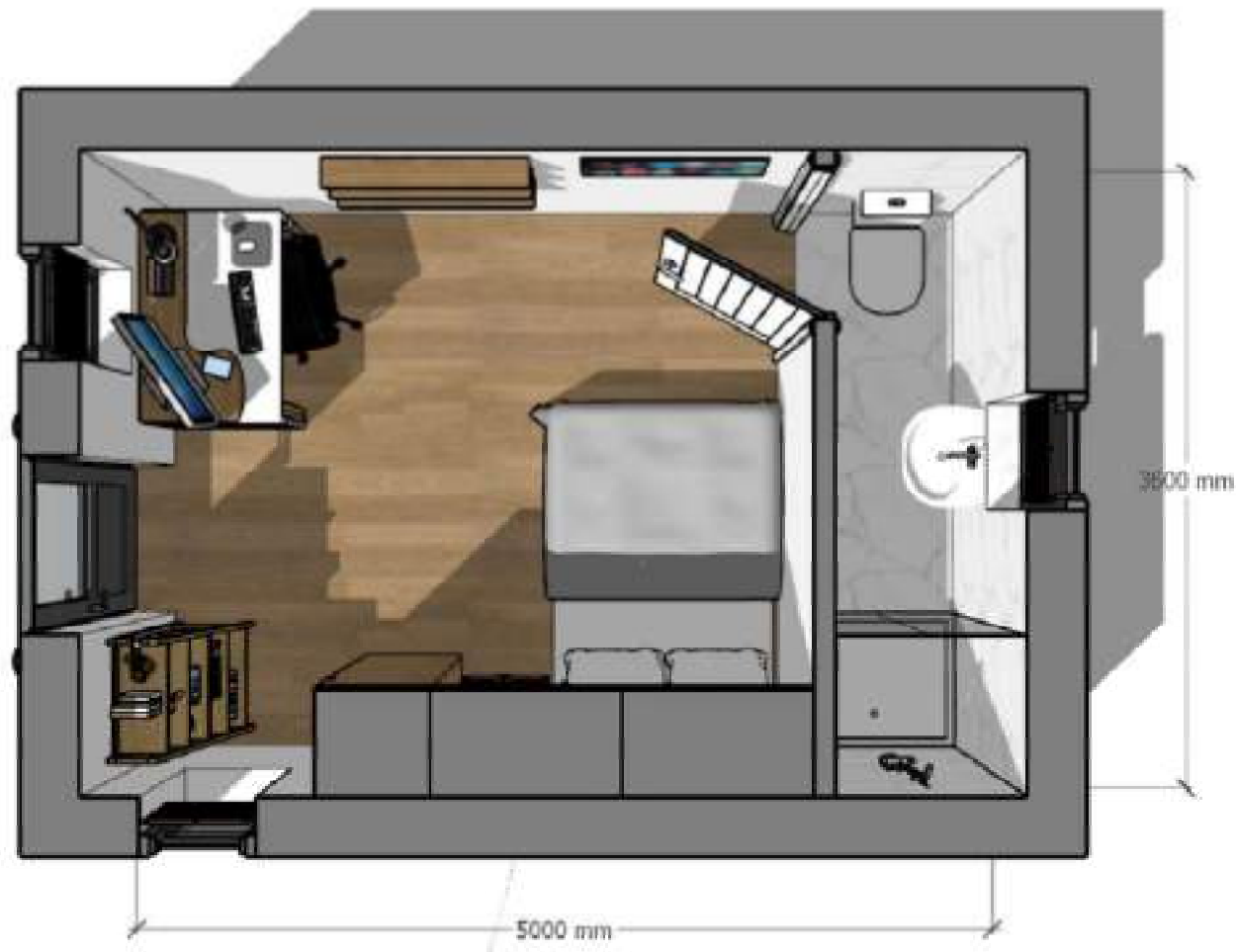
FLOOR PLAN 01 – FURNITURE LAYOUT (EXAMPLE ONLY)
