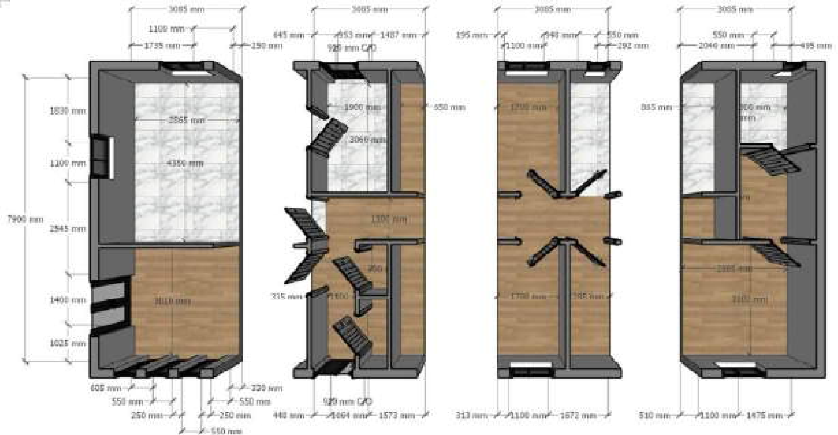
SECTION PLAN
