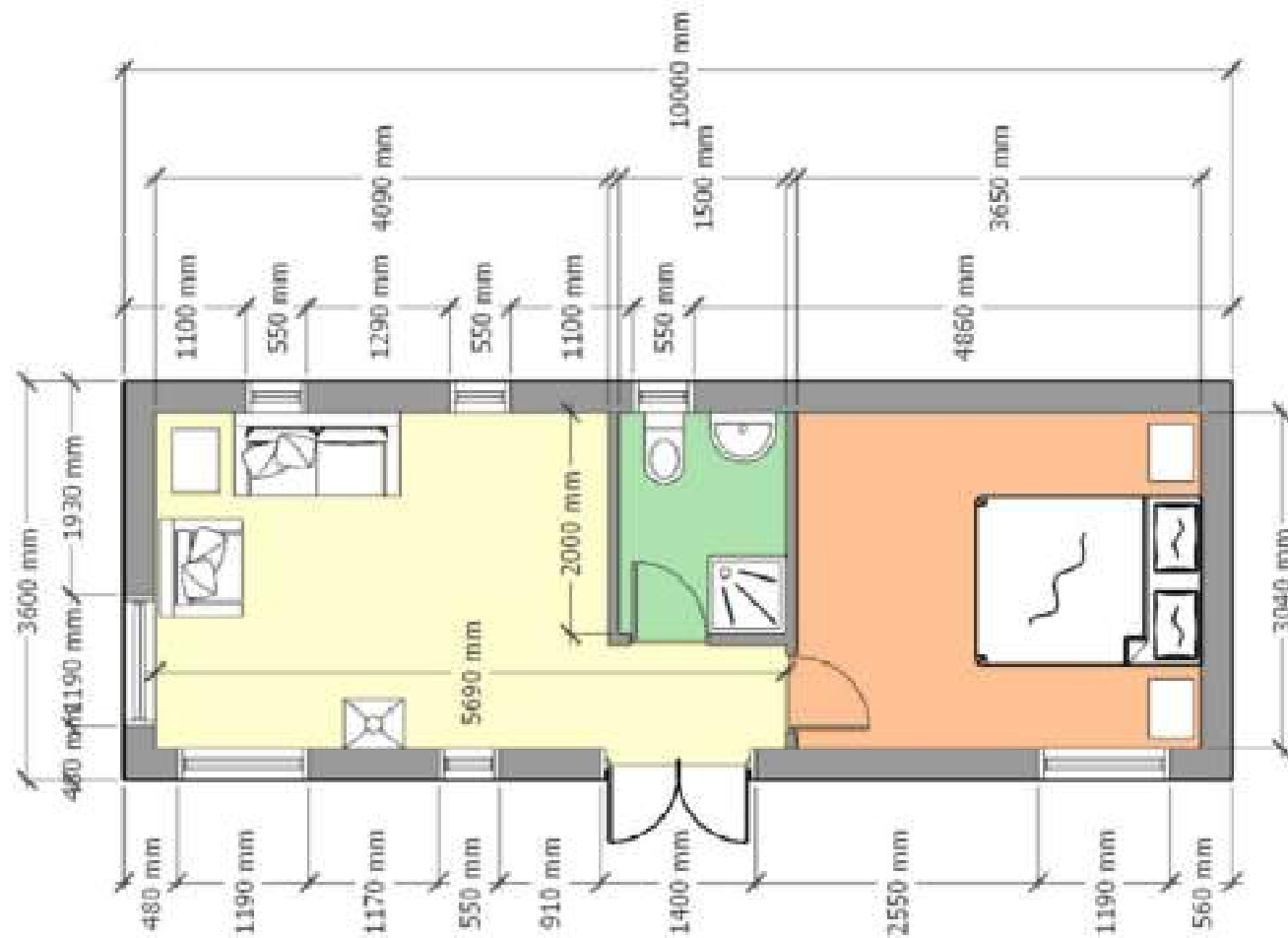
FLOOR PLAN 03 – EXTERNAL &amp; INTERNAL DIMENSIONS
