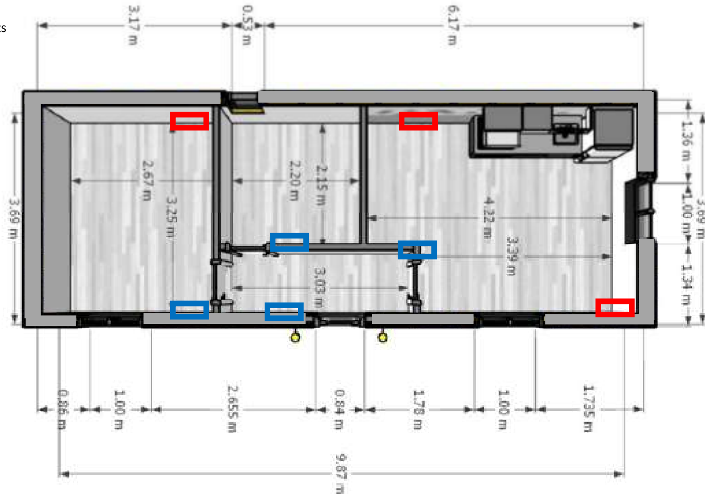
FLOOR PLAN 01 – SOCKET & SWITCHES
