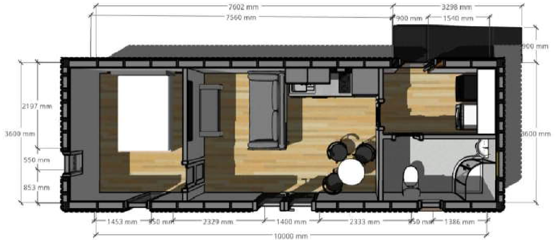
FLOOR PLAN 02
