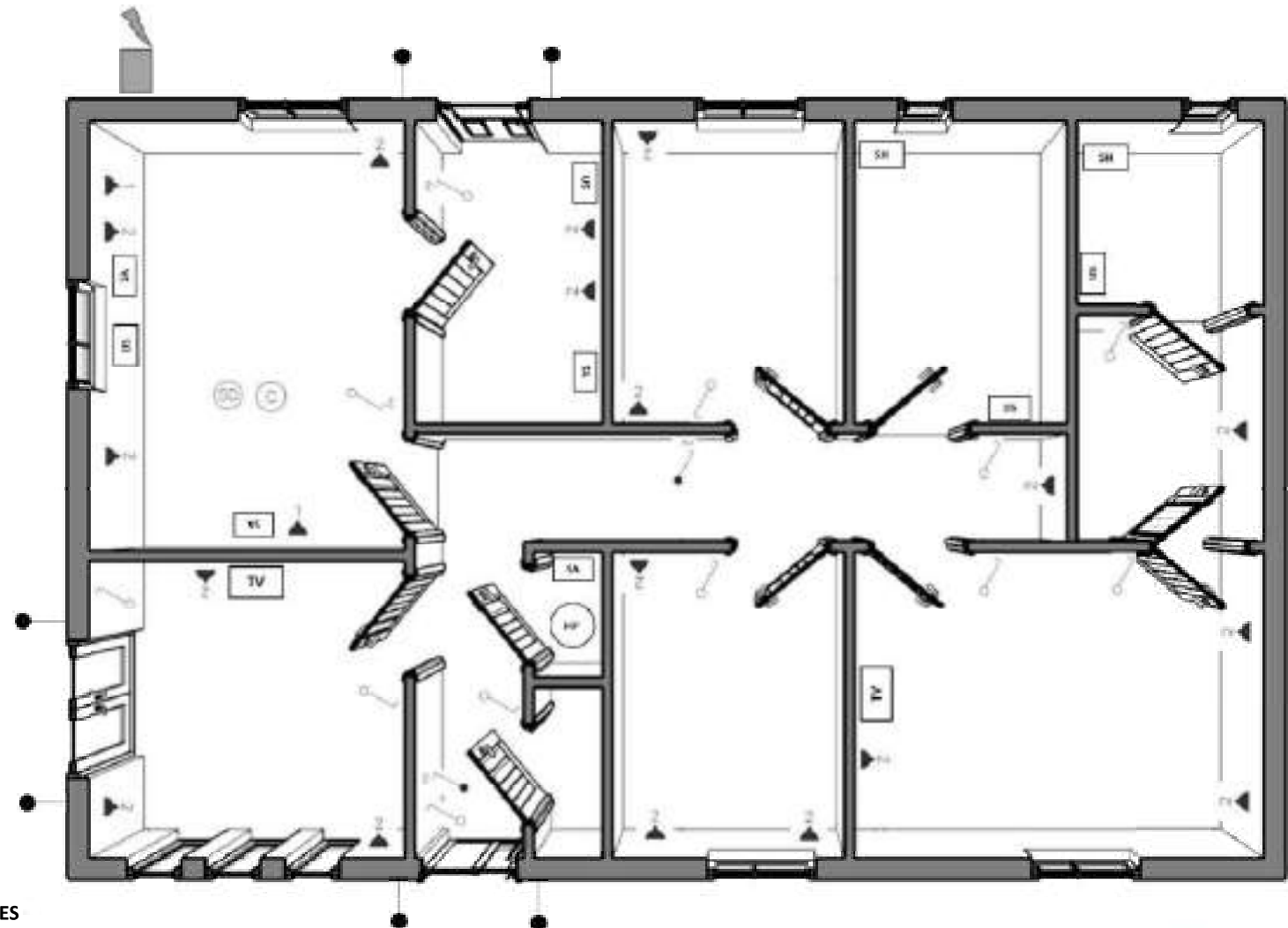
ELECTRICAL LAYOUT
