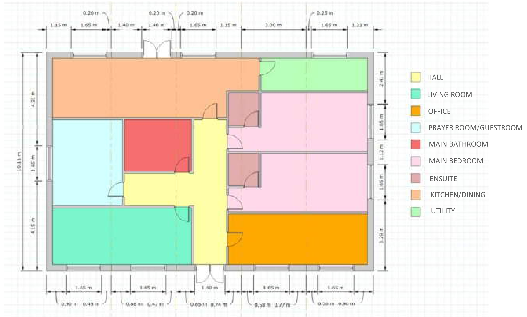
FLOOR PLAN 04 – MODULE DIMENSIONS
