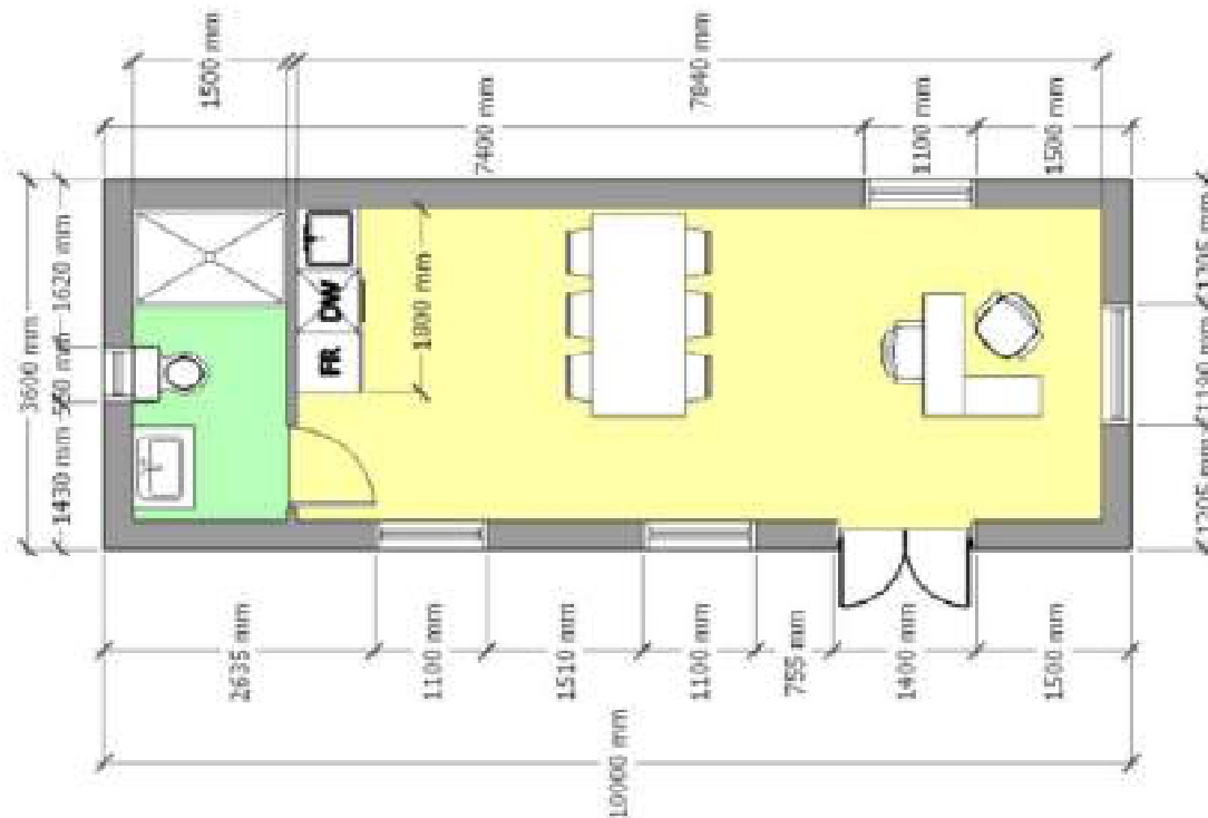
FLOOR PLAN 01
