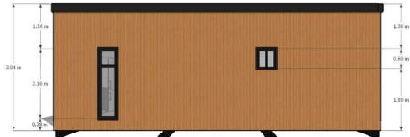
REAR ELEVATION
