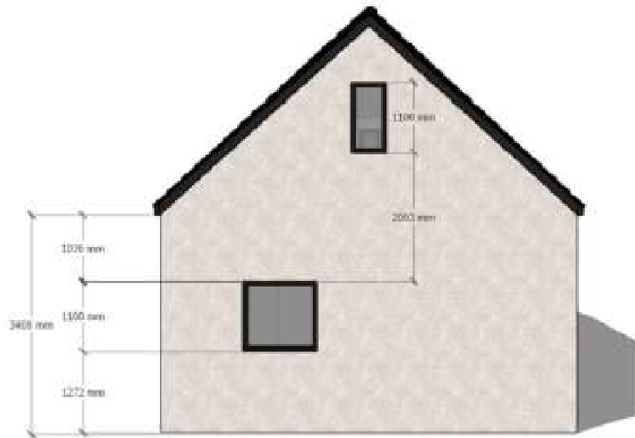
LHS ELEVATION
