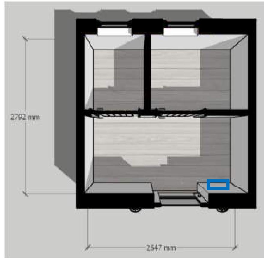
FLOOR PLAN 01 – SOCKET & SWITCHES
