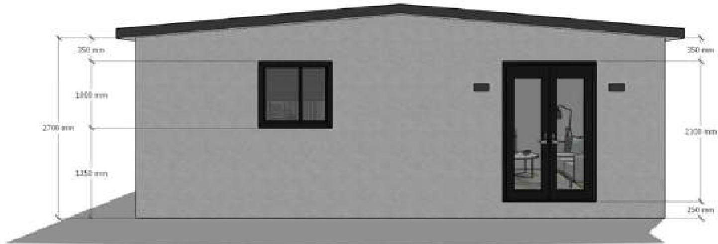
LHS ELEVATION
