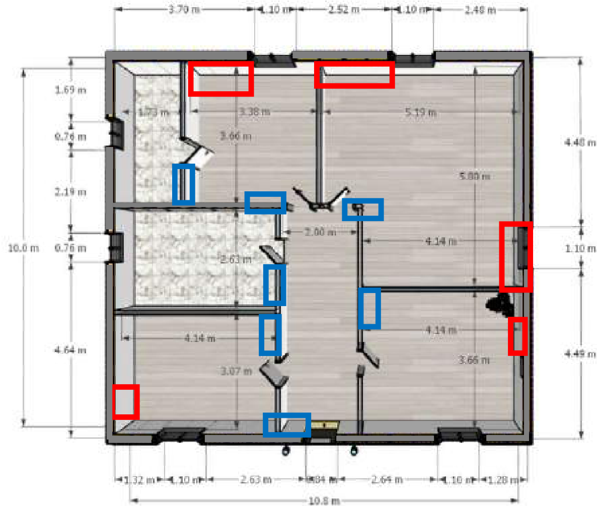
FLOOR PLAN 01 – SOCKET & SWITCHES
