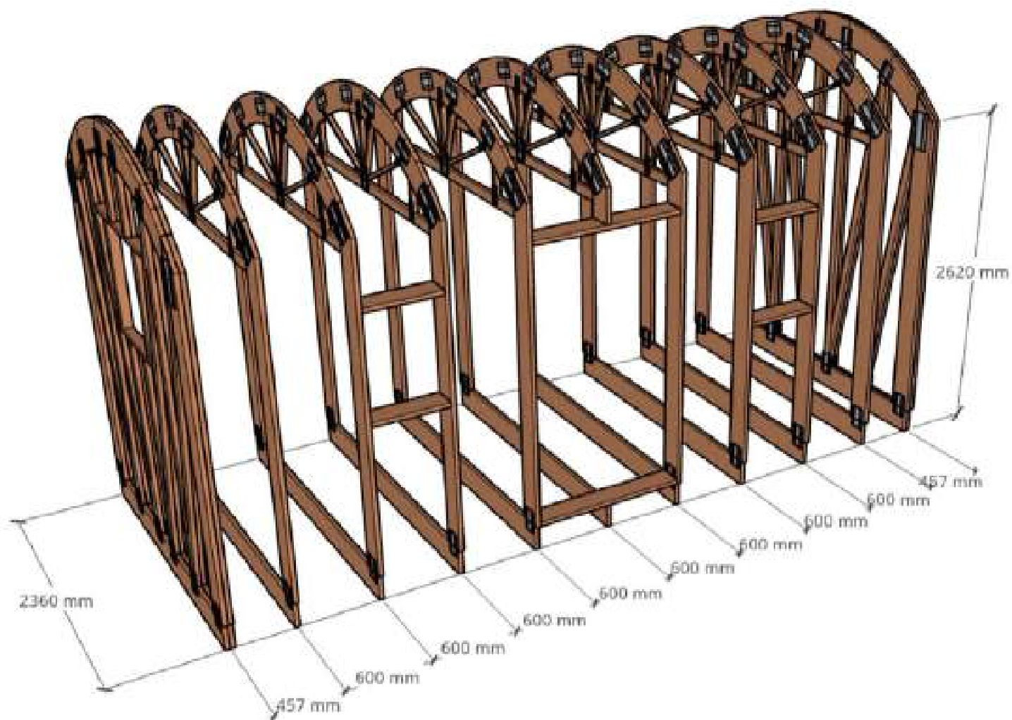
PROPOSED FRAME SETTING OUT
