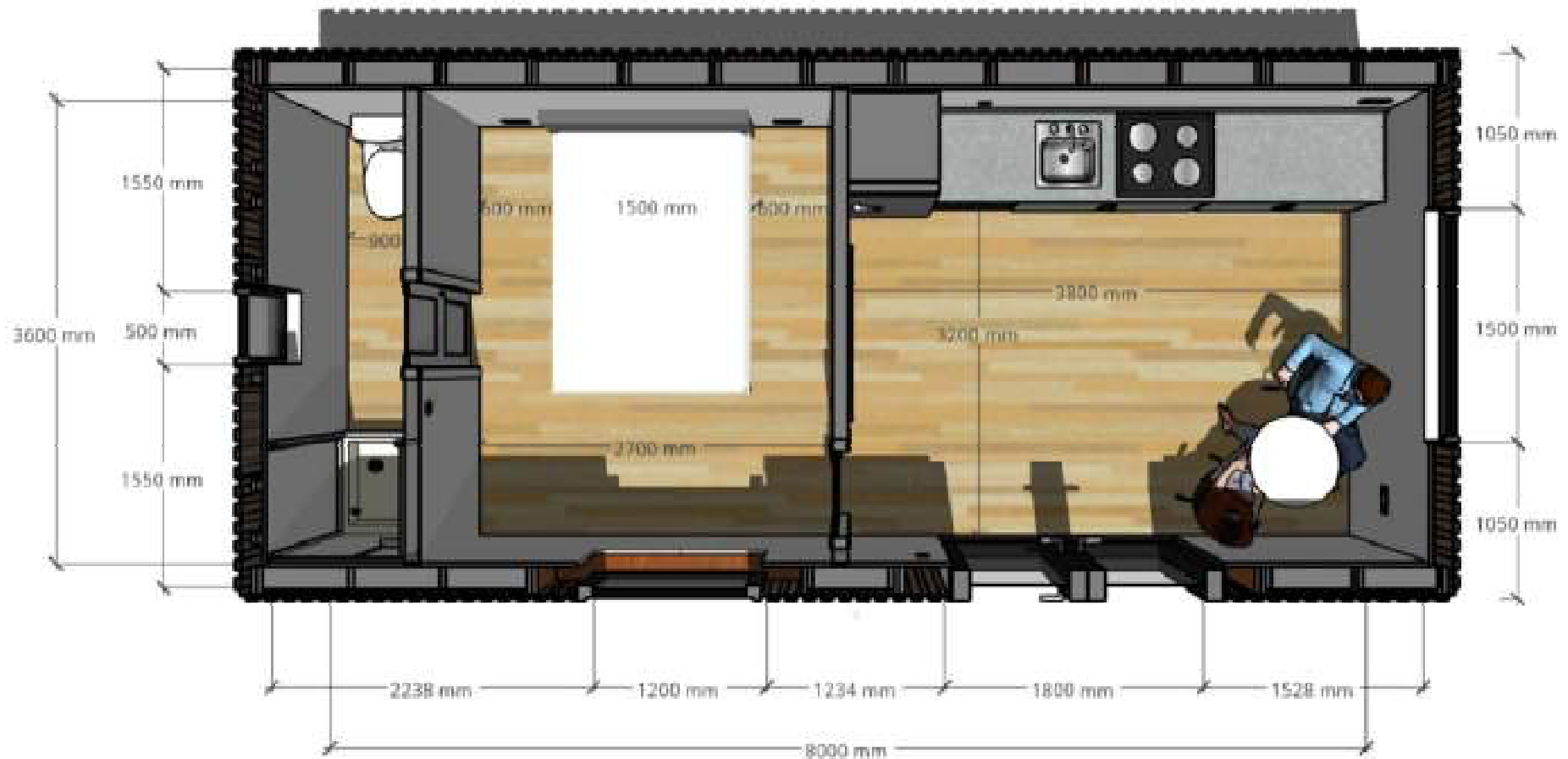
FLOOR PLAN 02
