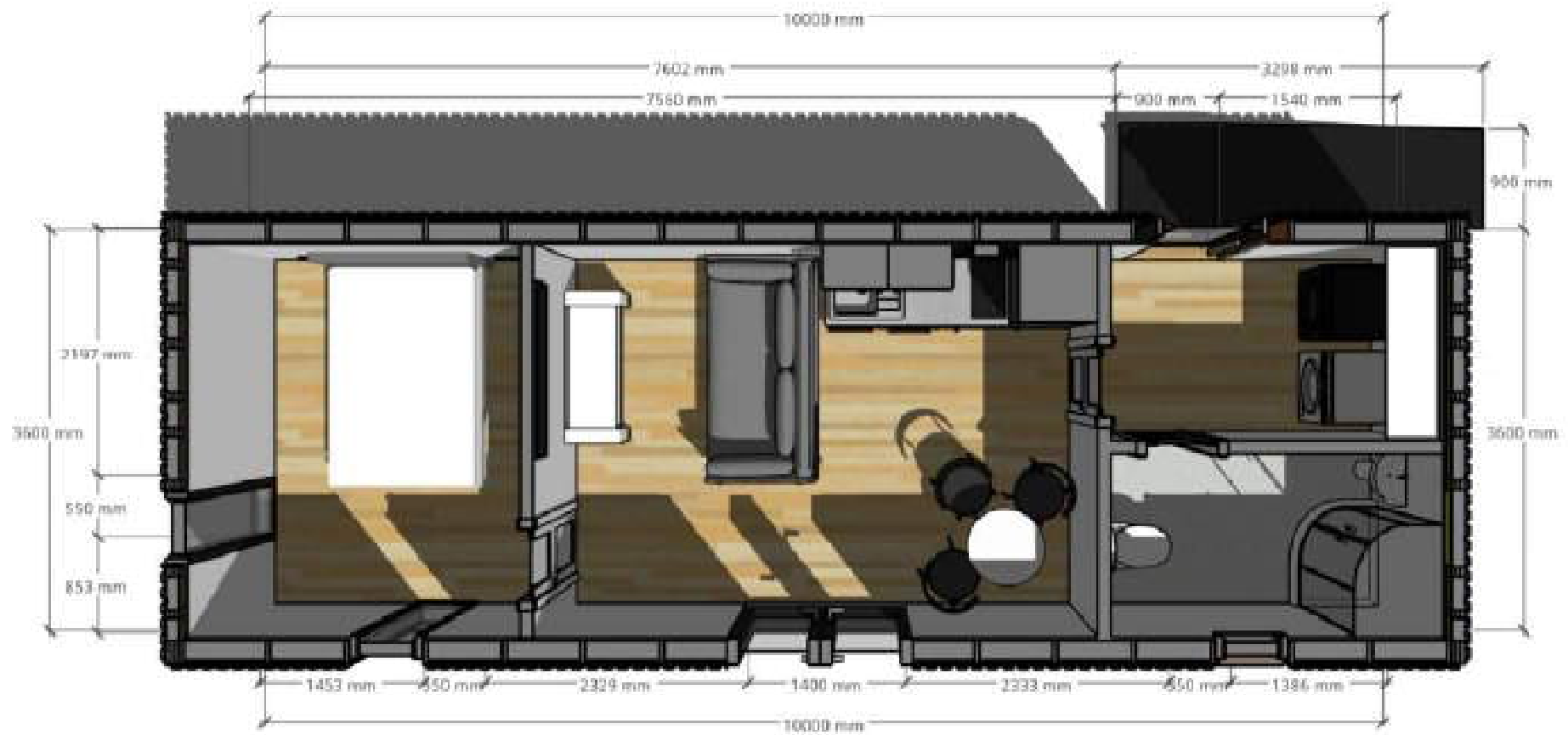
FLOOR PLAN 02
