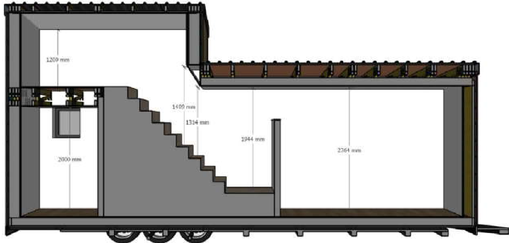
SECTION C-C
