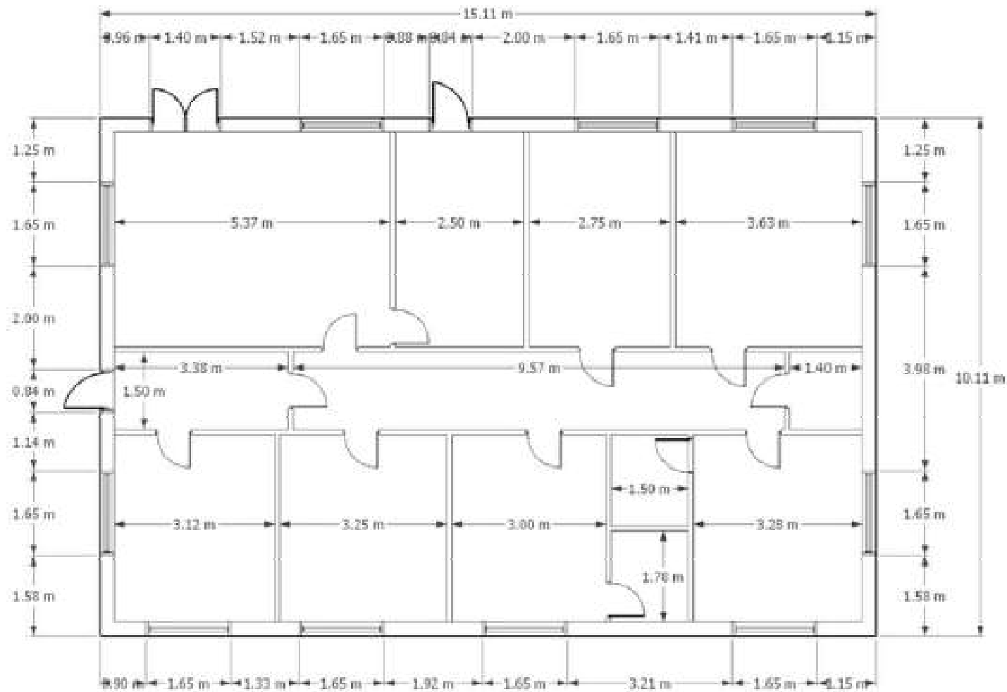
FLOOR PLAN 03 – EXTERNAL &amp; INTERNAL DIMENSIONS
